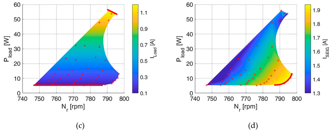
Figure 18. Load curves as a function of rotational speed and system boundary operation zone for C=16\mu F : (a) rectified voltage, (b) DC motor armature current, (c) load current and (d) SEIG current.
