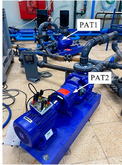
Figure 3. Pump as turbines used: PAT1 rated for 1050 rpm, and PAT2 rated for 760 rpm.
