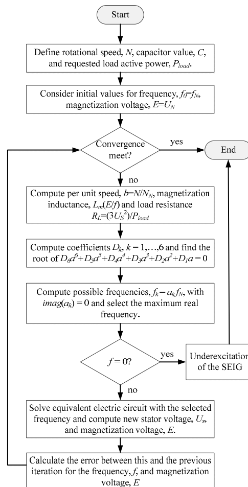
Figure 13. Flowchart describing the analytical procedure.
