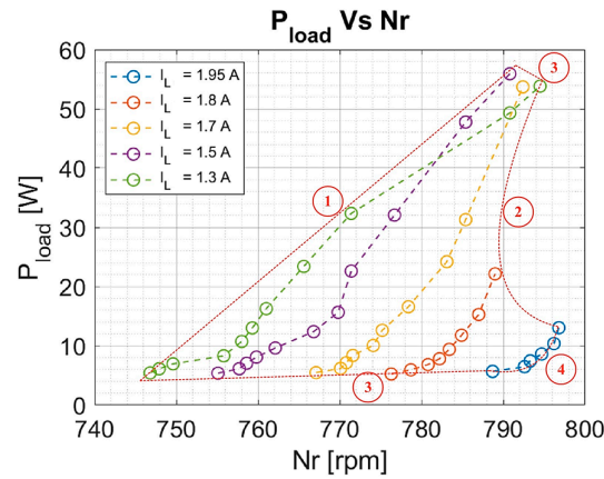
Figure 17. System load curve as a function of SEIG rotation speed for C=16\mu F .
