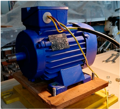
Figure 5. Induction Machine used as SEIG.
