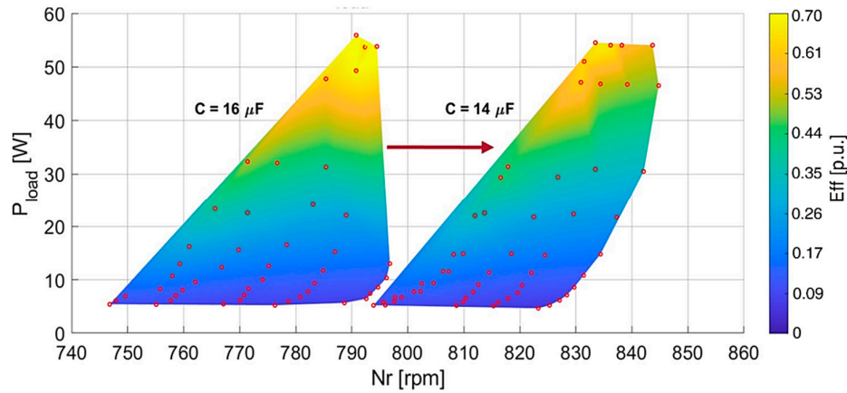
Figure 20. Comparison between the efficiency maps for C=16 \mu\text{F} and C=14 \mu\text{F} . 1 p.u. corresponds to 40%.
