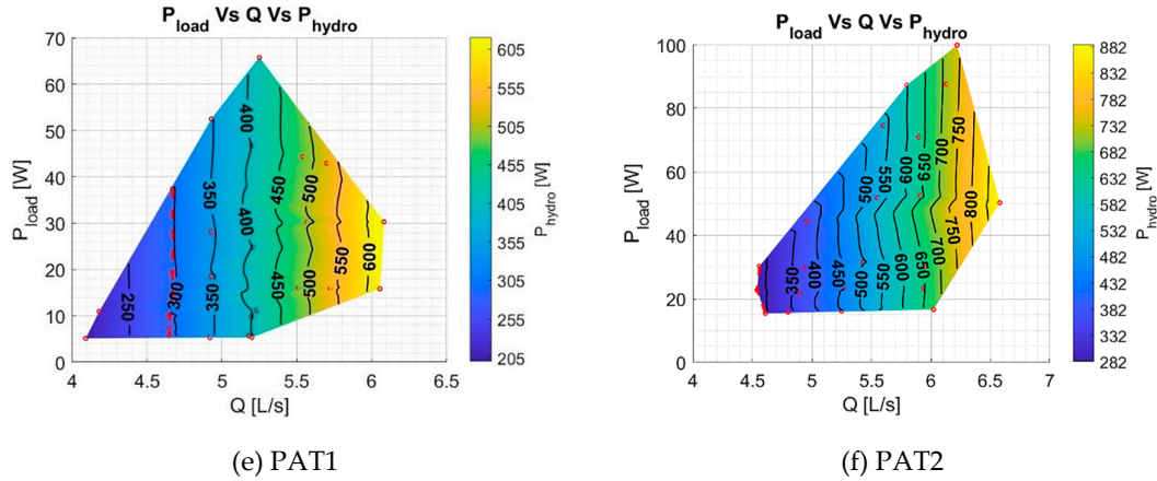
Figure 22. Influence on the hydraulic parameters for increasing loads, as a function of the load, P_{load} , and water flow, Q : (a) and (b) rotational speed, N_r , (c) and (d) head, H , and (e) and (f) hydraulic power, P_{hydro} , for PAT1 and PAT2.
