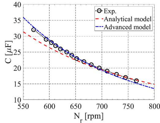
Figure 15. Required capacitor value to self-excite the induction machine for different speeds. Experimental tests in 'o', the analytical model (2) in red and the advanced model [26] in blue.
