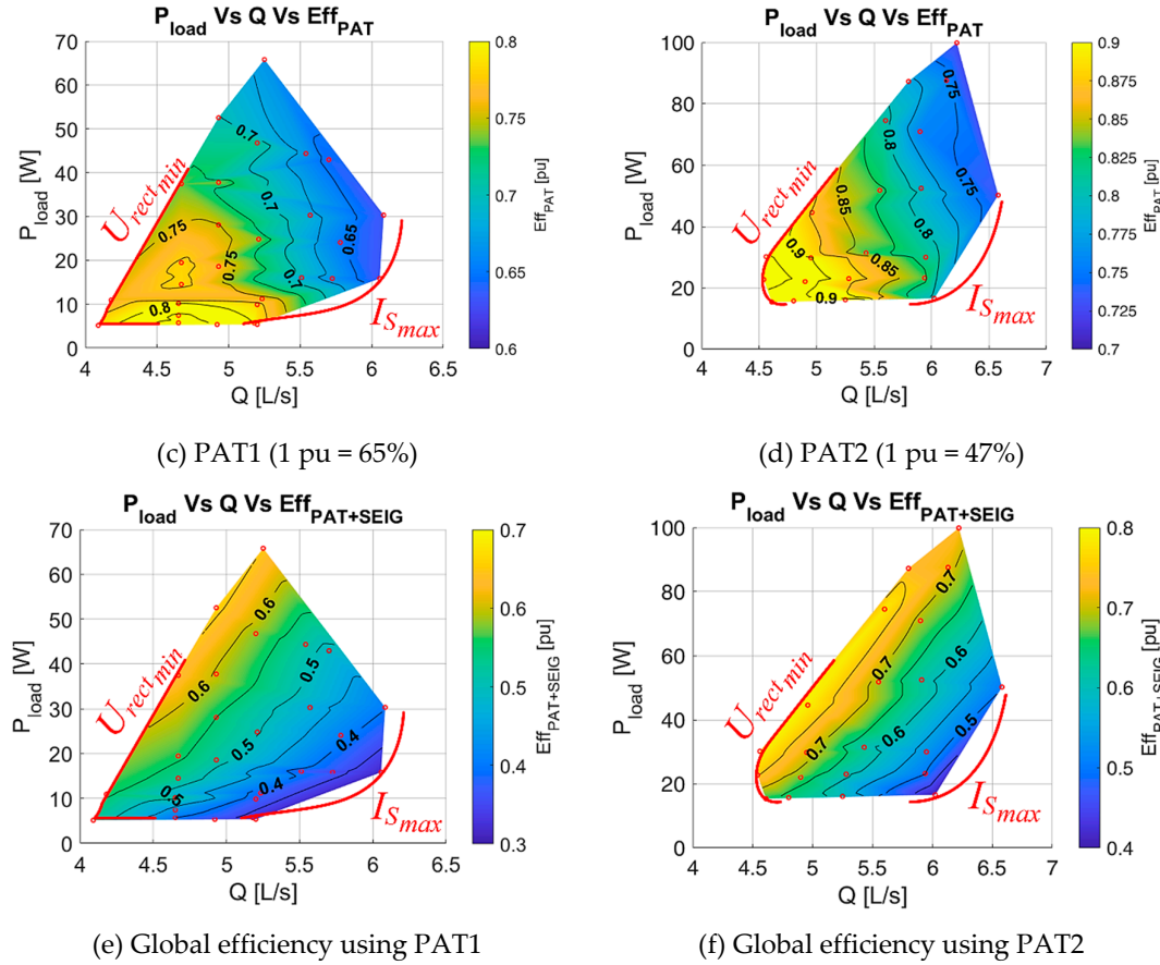
Figure 23. System's efficiency as a function of the load, P_{load} , and water flow, Q : (a) and (b) SEIG efficiency, (c) and (d) PAT efficiencies, and (e) and (f) global efficiency for PAT1 and PAT2.
