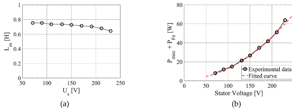
Figure 14. Magnetizing Inductance and mechanical and iron losses as a function of the stator voltage.
