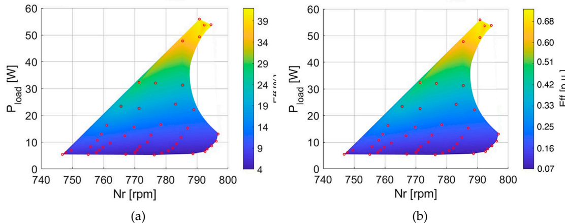
Figure 19. Efficiency map of the electric system for C=16\mu F : (a) absolute values of efficiency and (b) efficiency per unit values referred to the SEIG nominal efficiency.
