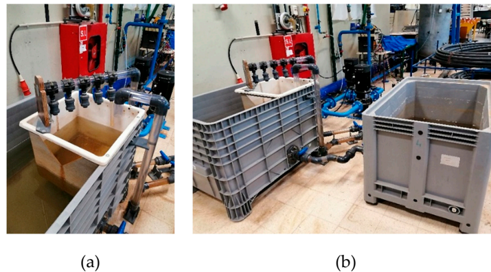
Figure 10. Downstream reservoir inserted in the buffer to ensure a pressure drop at the PAT and a closed loop system.
