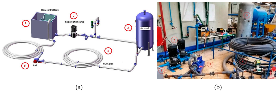
Figure 9. Hydraulic system to be used to test the electric system: 1) flow control tank, 2) recirculating pump, 3) Air-vessel, 4) pipes and 5) PAT coupled to the SEIG.
