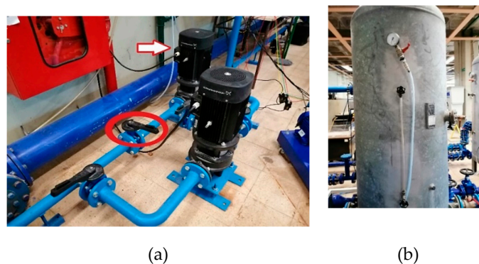
Figure 11. Pumps to feed water from the buffer to the air-vessel reservoir(a). Air vessel (or hydropneumatics) reservoir connected to an air pressure control valve to allow pressure and flow variation at the PAT input (b).
