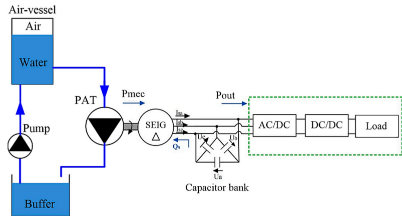
Figure 2. DC off-grid composed by a PAT-SEIG system.
