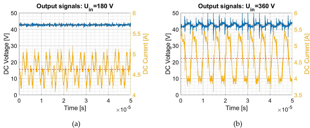
Figure 16. DC/DC output voltage for two input voltage values and for a load of 200W.
