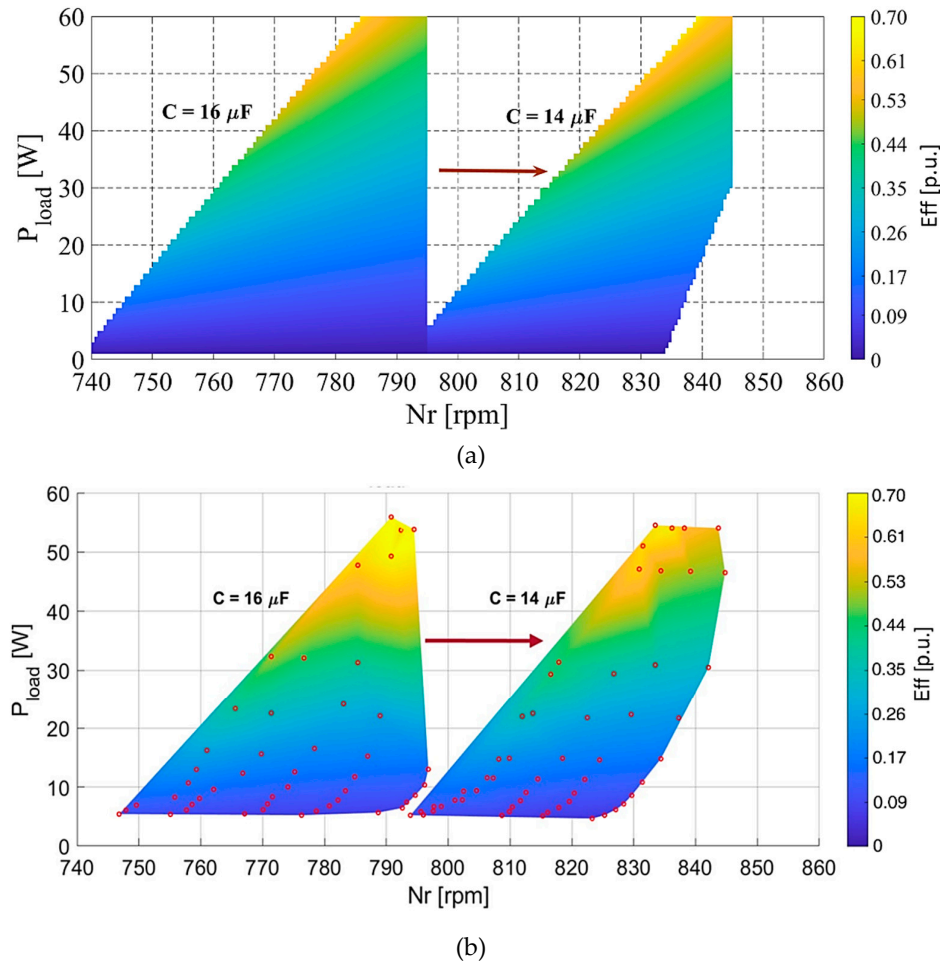
Figure 24. Comparison between analytical (a) and experimental results (b) applied for the same range of rotational speed and load of the SEIG.
