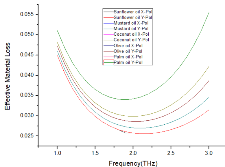
Figure 7. The EML variation with frequency for different oil samples over the frequency ranging from 1.0 to 3.0 THz.
