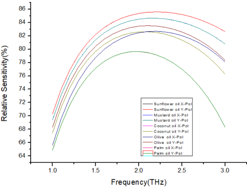
Figure 6. The relative sensitivity variation with frequency for different oil samples over the frequency ranging from 1.0 to 3.0 THz.
