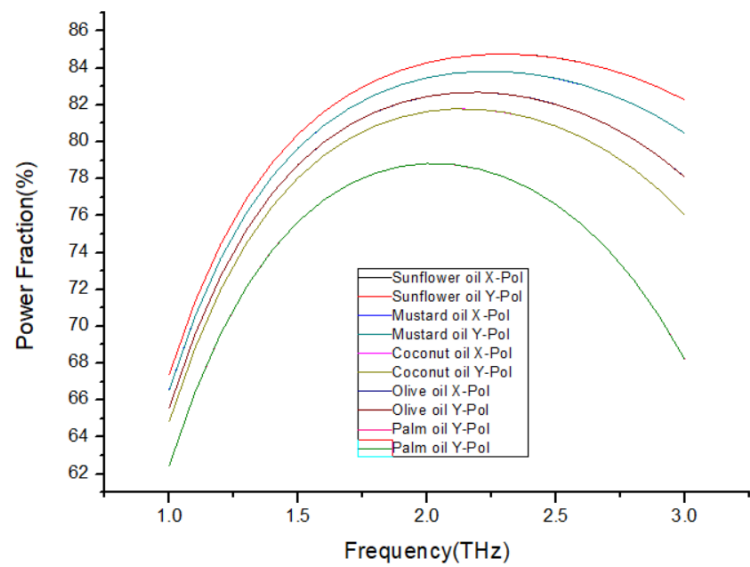
Figure 9. The Power Fraction variation with frequency for different oil samples over the frequency ranging from 1.0 to 3.0 THz.
