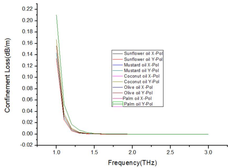
Figure 8. The CL variation with frequency for different oil samples over the frequency ranging from 1.0 to 3.0 THz.
