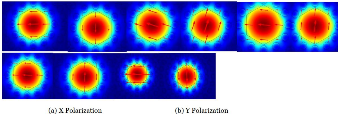
Figure 5. Light mode distribution of PCF-based oil detection of Proposed sensor.
