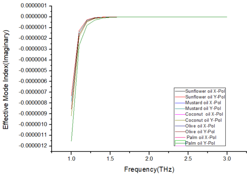
Figure 12. Change of effective refractive index(imaginary) with increasing frequency from 1.0 to 3.0 THz for different oil samples.
