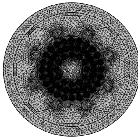
Figure 3. Meshing output with boundary condition of the suggested sensor.
