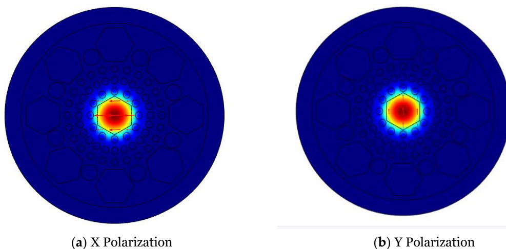
Figure 4. Light Confinement in the PCF-based oil detection of the Proposed sensor's core.
