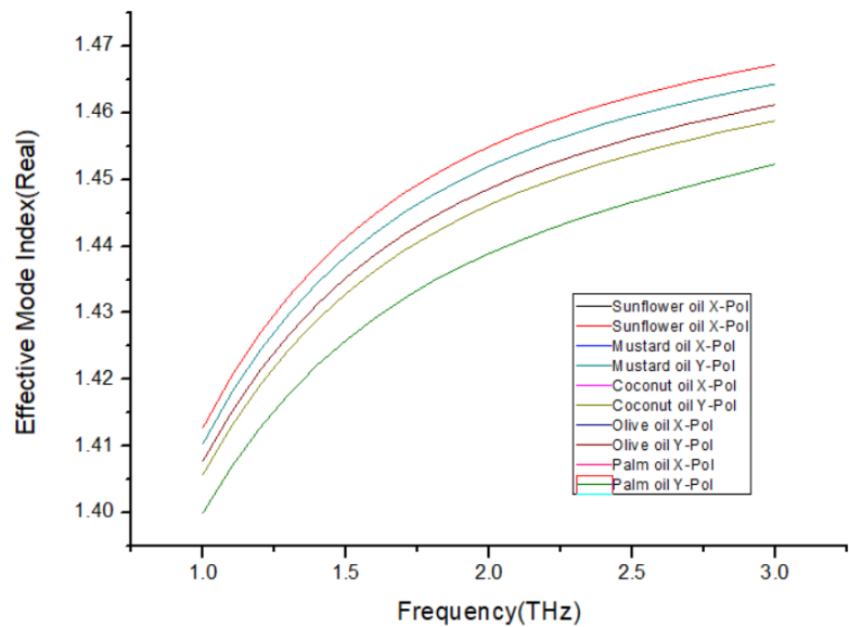
Figure 11. Change of effective refractive index(real) with increasing frequency from 1.0 to 3.0 THz for different oil samples.
