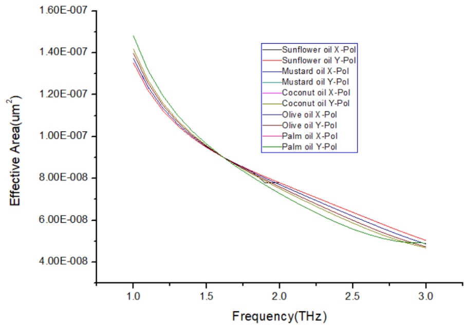
Figure 10. The effective area variation with frequency for different oil samples over the frequency ranging from 1.0 to 3.0 THz.
