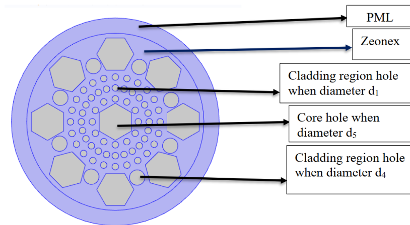
Figure 2. Designed view of proposed Hollow Core-Based PCF edible oil detection sensor in two dimensions.
