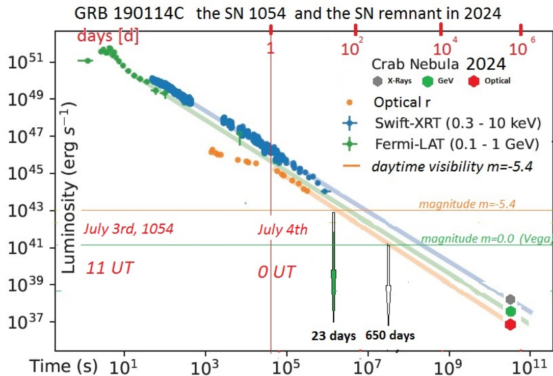
Figure 1. The light-curve of the GRB 190114C extrapolated for 10^3 years or 3\cdot10^{10} s.
