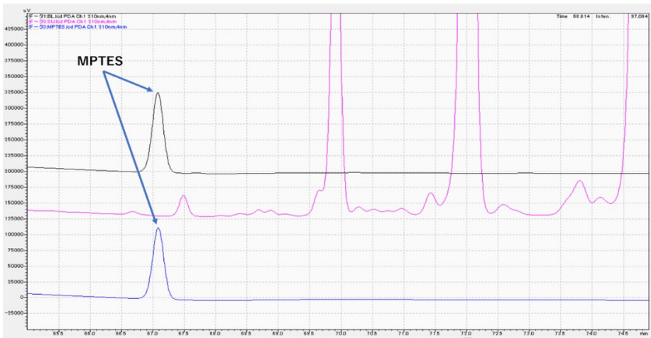
Figure 2. HPLC chromatogram expanded from 65 to 75 minutes. Tokuyama Universal Bond II (black), Scotchbond Universal Plus Adhesive (pink) and MPTES (blue).
