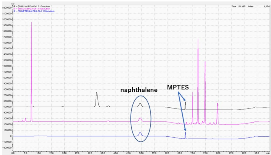
Figure 1. High-performance liquid chromatography (HPLC) results of Tokuyama Universal Bond II (black), Scotchbond Universal Plus Adhesive (pink) and 3-(triethoxysilyl)propyl methacrylate (MPTES) (blue).
