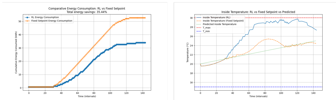
Figure 10. Energy Consumption: RL vs Fixed Setpoint (left) and Inside Temperature: RL vs Fixed Setpoint vs Predicted (right)
