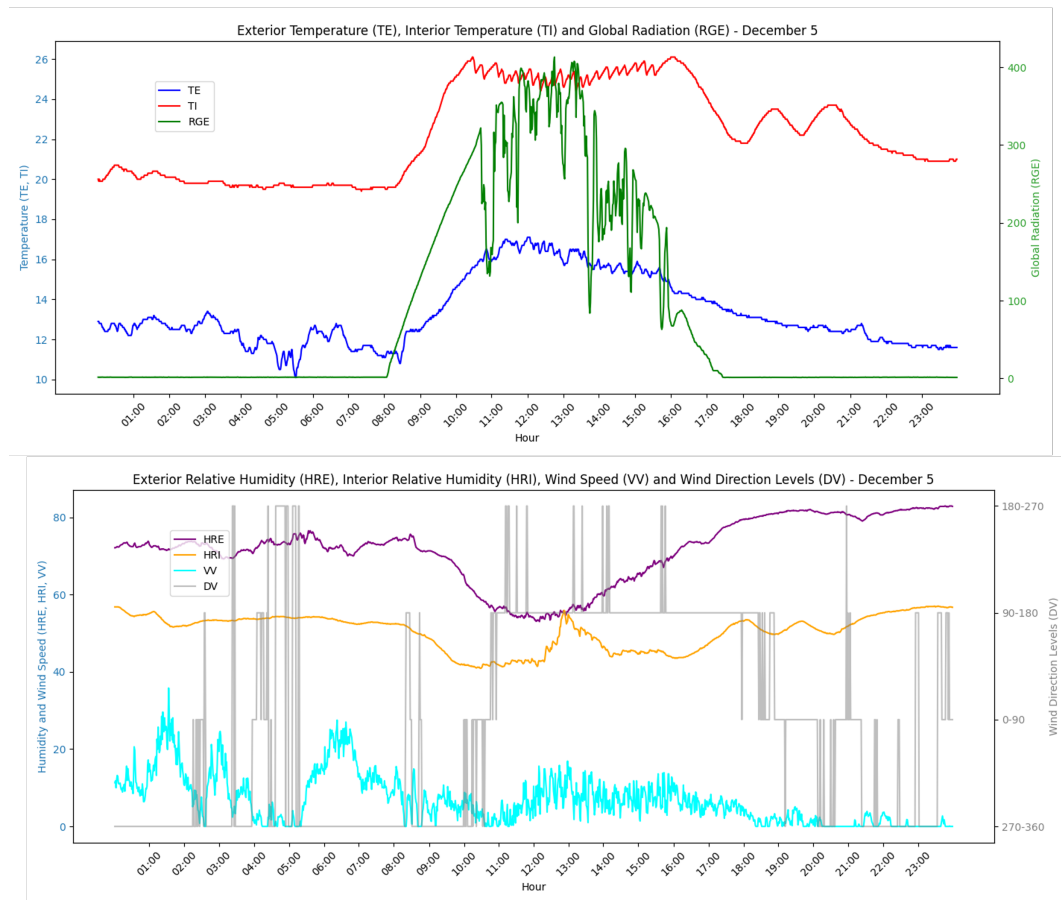
Figure 5. Example of daily data obtained in the dataset. The data is obtained daily every minute and stored in a dataset to obtain temperature prediction models inside the greenhouse.
