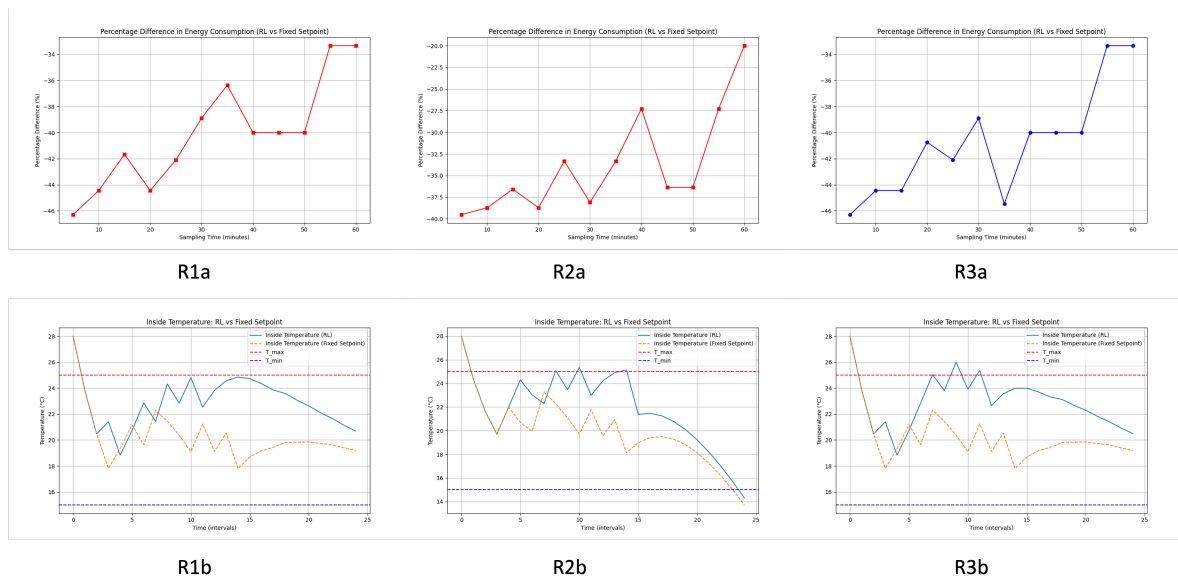
Figure 7. Comparative analysis in greenhouse cooling process
