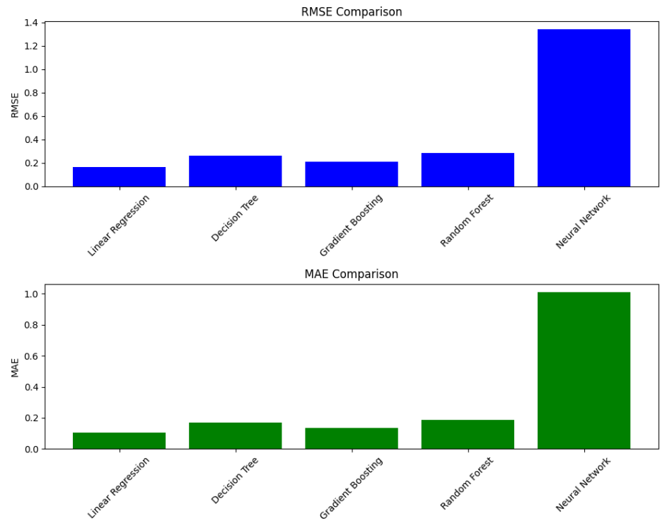
Figure 9. Machine learning methods to predict the temperature inside the greenhouse ( TI )
