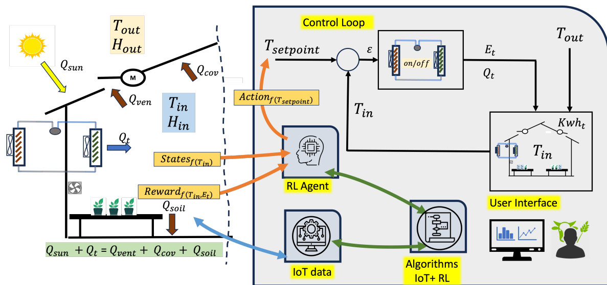
Figure 1. RL paradigm in greenhouse proposed
