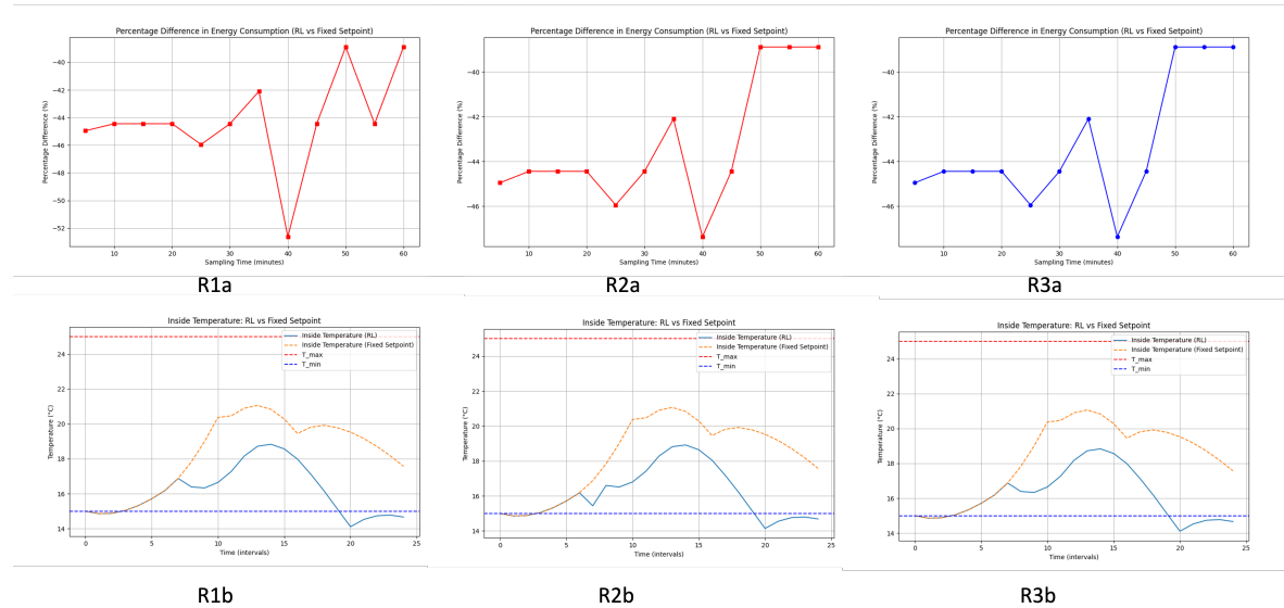
Figure 8. Comparative analysis in greenhouse heating process
