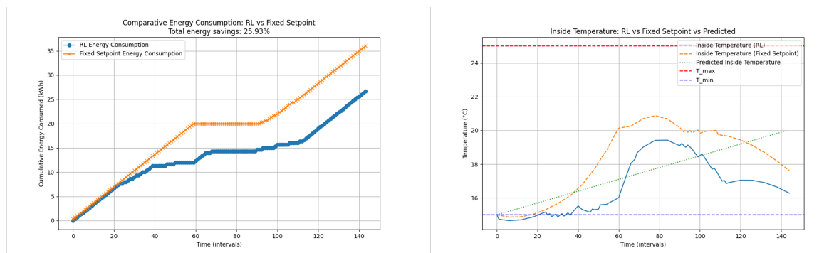
Figure 11. Comparative Energy Consumption: RL vs Fixed Setpoint and Inside Temperature: RL vs Fixed Setpoint vs Predicted
