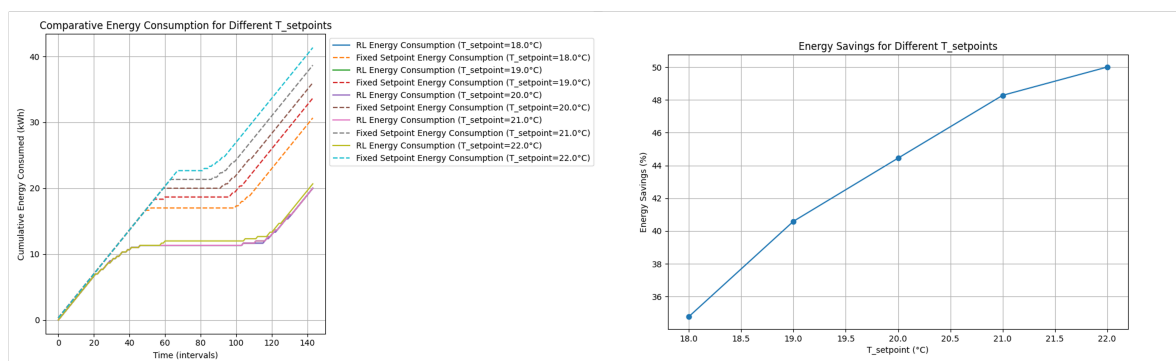
Figure 12. Comparative analysis taking different reference temperatures (setpoints)
