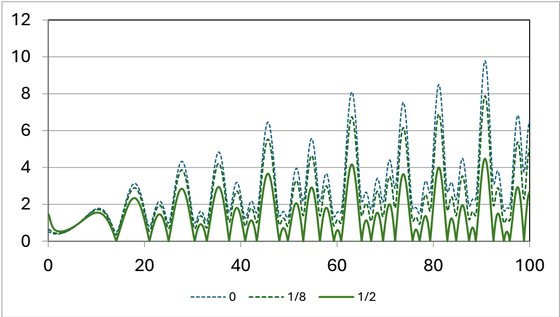
Figure 2. Plots of |\zeta(\sigma + it)| with \sigma = \left\{0, \frac{1}{8}, \frac{1}{2}\right\} and 0 \leq t \leq 100 .
