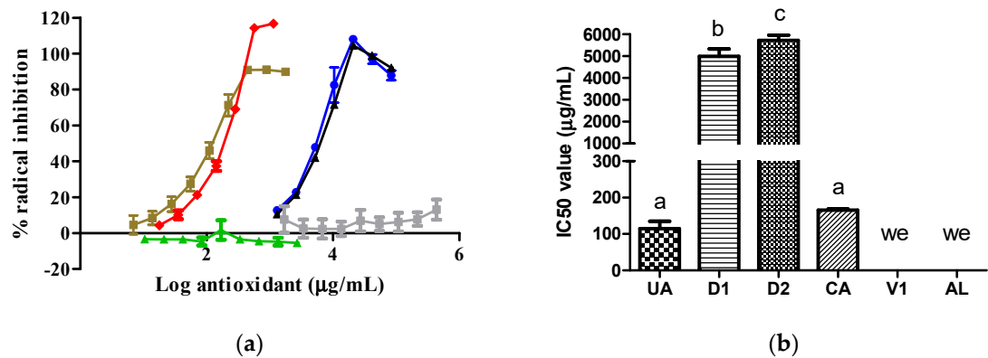
Figure 3. Activity of samples against the DPPH radical: (a) DPPH radical inhibition graph; (b) IC50 values calculated from curves. In Figure 3b, the lowercase letters a, b, and c above the bars indicate statistical differences ( p < 0.0001 ). The green, red, gray, blue, black, and brown lines represent the AL, CA, V1, D1, D2, and UA samples, respectively. we, with no effect. DPPH, 2,2'-diphenyl-1-picrylhydrazyl. CA and V1 data were collected from a prior evaluation [5].
