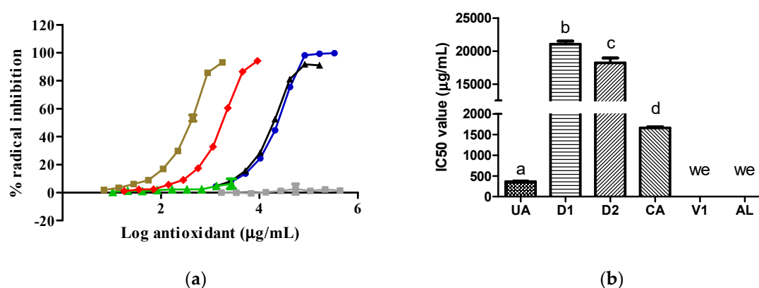
Figure 2. Activity of samples against the ABTS radical: (a) ABTS radical inhibition graph; (b) IC 50 values calculated from curves. In Figure 2b, the lowercase letters a, b, and c above the bars indicate statistical differences ( p < 0.0001 ). The green, red, gray, blue, black, and brown lines represent the AL, CA, V1, D1, D2, and UA samples, respectively. we, with no effect. ABTS, 2,2'-azino-bis 3-ethylbenzothiazoline-6-sulfonic acid; UA, uric acid. CA and V1 data were collected from a prior evaluation [5].
