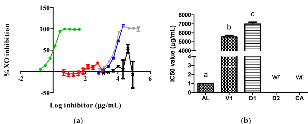
Figure 1. Activity of samples against the XO enzyme: (a) XO inhibition graph; (b) IC 50 values calculated from curves. In Figure 1b, the lowercase letters a, b, and c above the bars indicate statistical differences ( p < 0.0001 ). The green, red, gray, blue, and black lines represent the AL, CA, V1, D1, and D2 samples, respectively. wr, with no concentration–inhibition relationship. XO, xanthine oxidase; AL, allopurinol; V1, vehicle.
