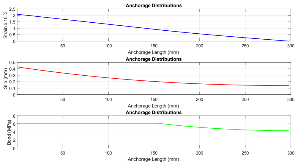
Figure 5. Strain, Slip and Bond distributions along the straight anchorage length of center shear-critical column of Specimen 2 for pushover step 15 of Phaethon Windows software. See also Figure 1 and 4. .
