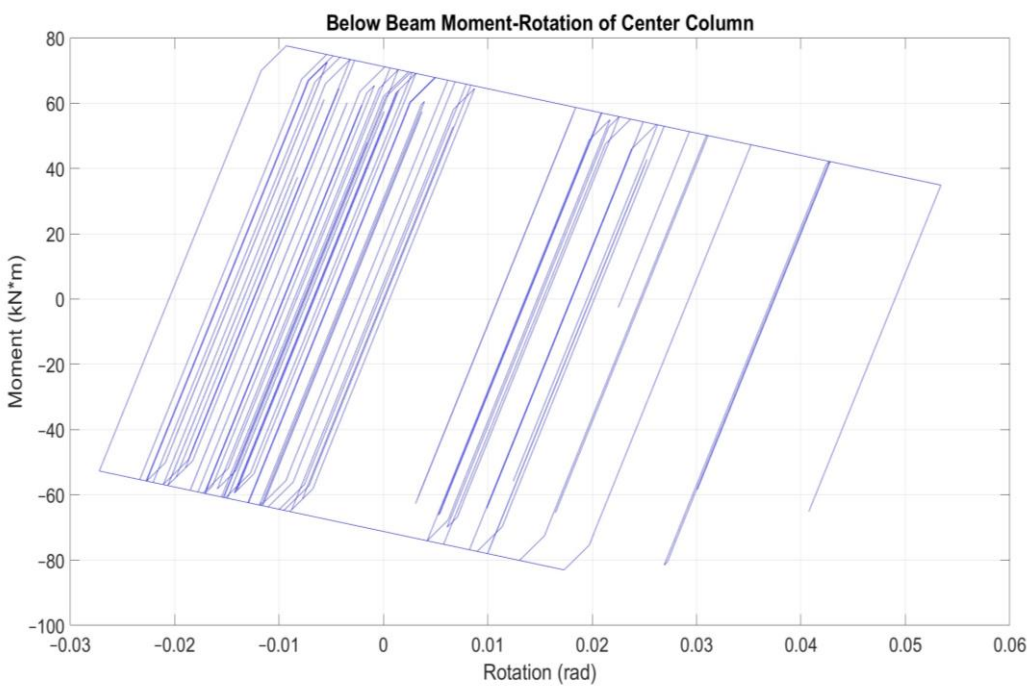
Figure 9. Below beam moment-rotation hysteretic response of center column of Specimen 2.
