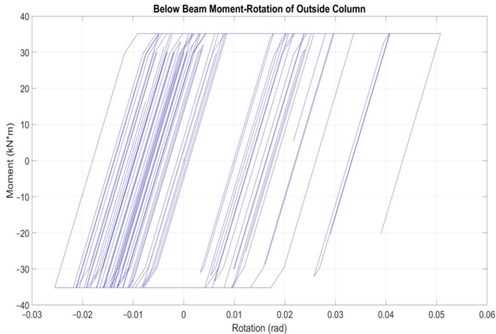
Figure 10. Below beam moment-rotation hysteric response of outside column of Specimen 2.
