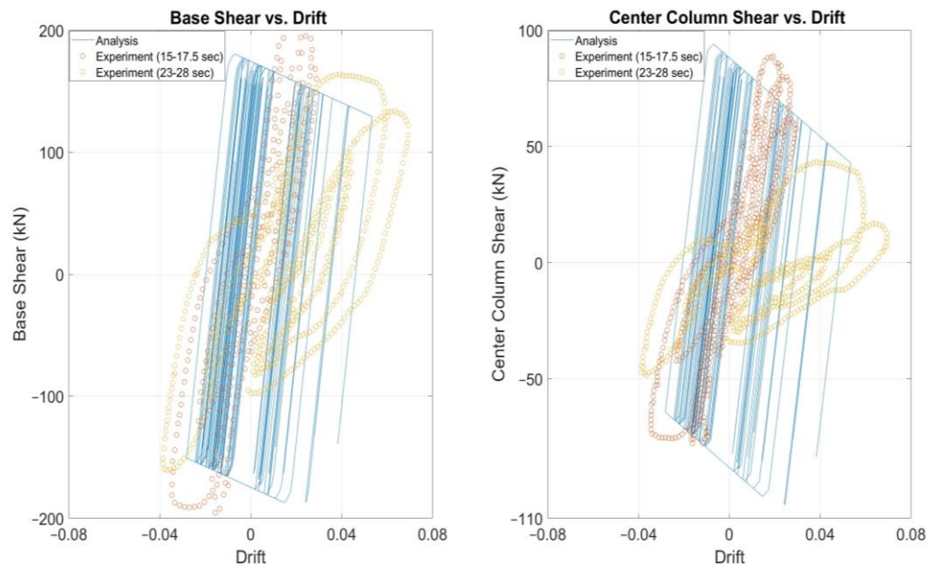
Figure 8. Shear hysteretic response of Specimen 2.
