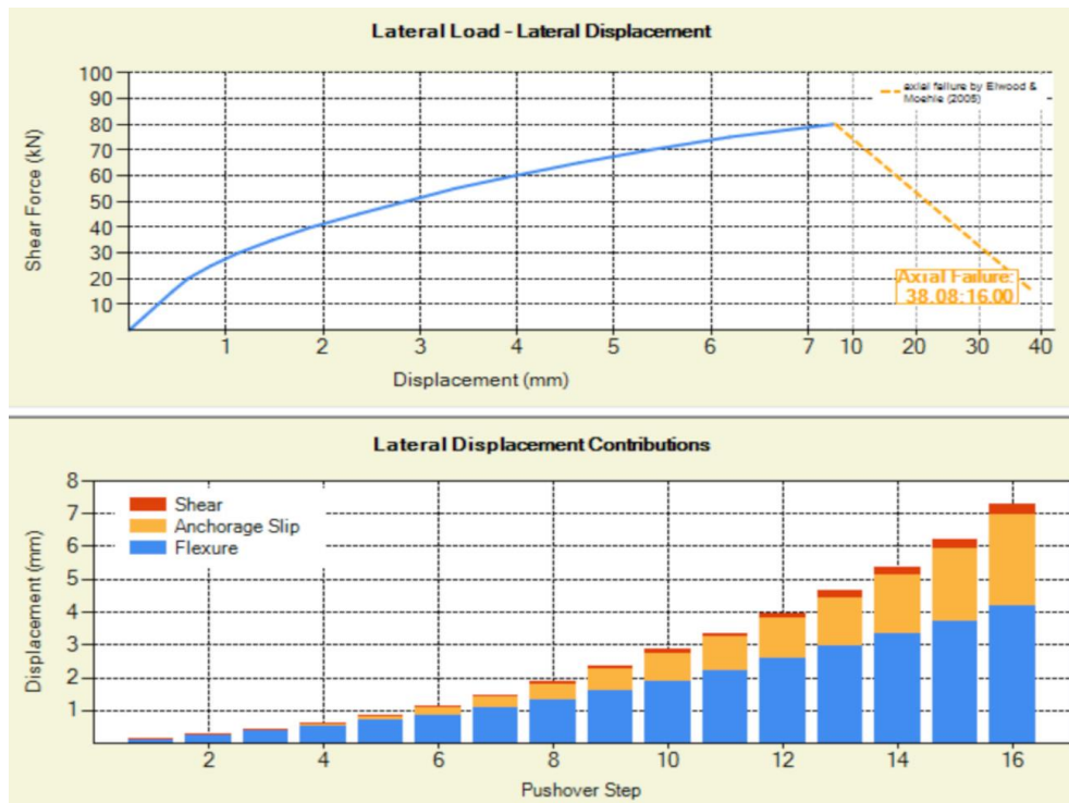
Figure 4. Capacity curve of center shear-critical column of Specimen 2 and lateral displacement contributions for each step of the pushover analysis (16 total pushover steps of 5 kN)[This is a screenshot from Phaethon Windows software user's interface].
