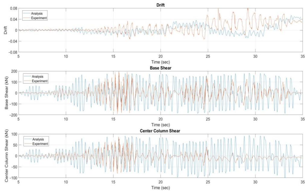
Figure 6. Time-history responses in terms of drift, base shear, and center column shear of Specimen 2.
